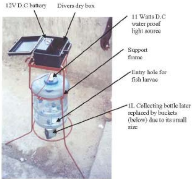
Plate 1 a: The locally fabricated light trap (a) showing optional collection buckets with trapped fish
