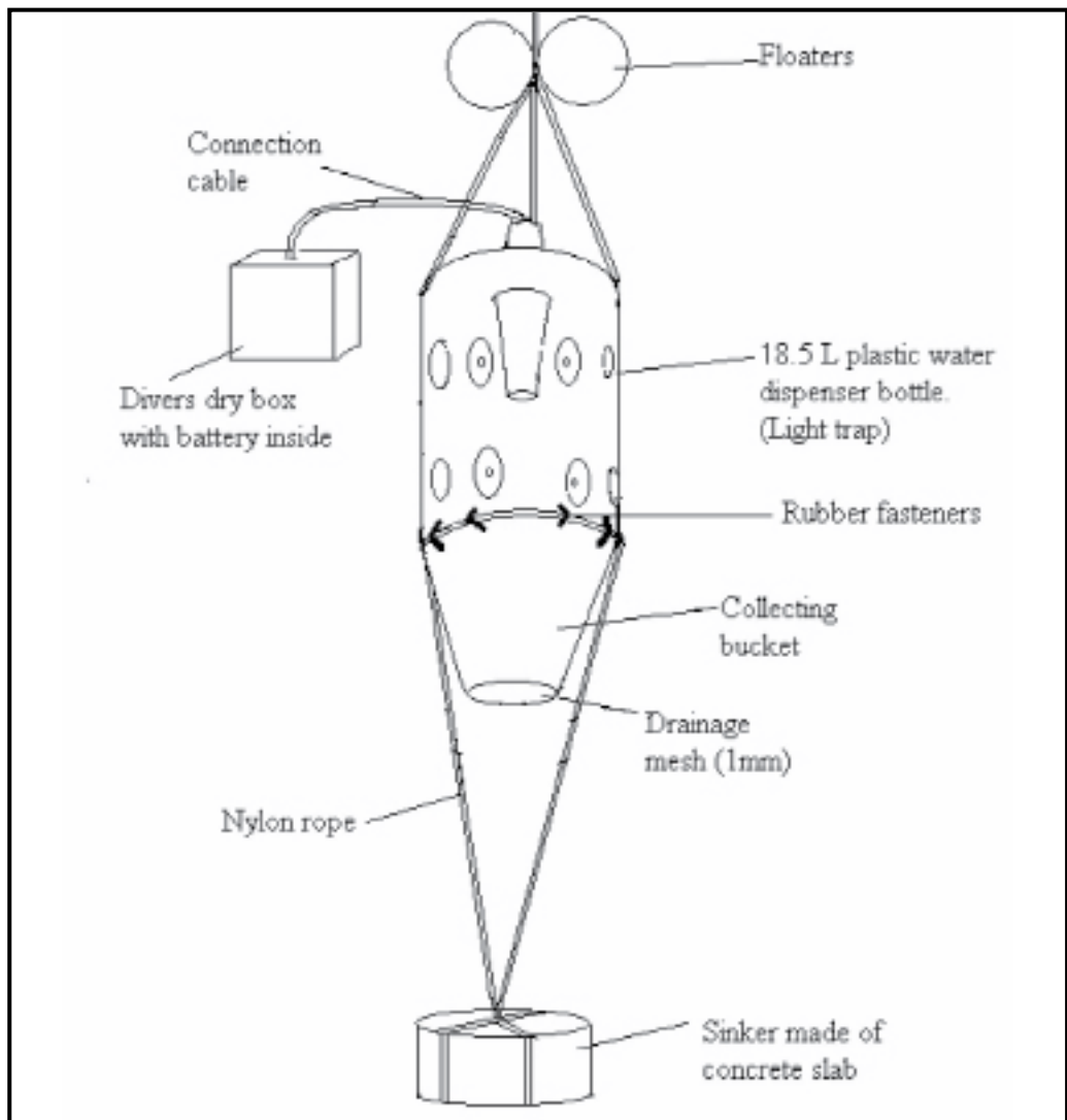
Fig. 1. Diagram of light trap without iron frame ready for deployment mid water. Floaters and a sinker ensure upright positioning of the light trap at desired depth
