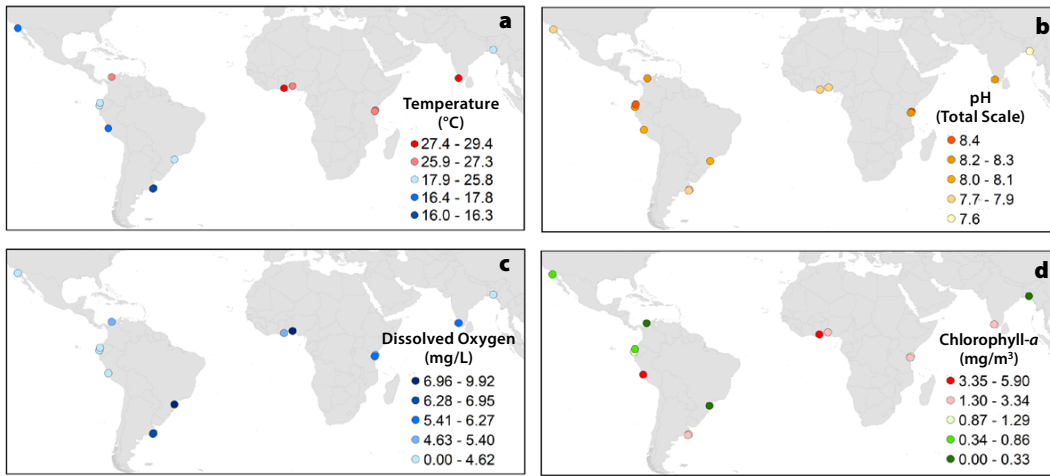
FIGURE 2. Average surface (0–10 m) Essential Ocean Variables: (a) temperature, (b) pH, (c) dissolved oxygen, and (d) chlorophyll- \alpha concentration sampled at NANO-DOAP stations. Time series vary from station to station, with the earliest sampling in December 2018 and the latest in September 2021. Stations in Argentina, Indonesia, Lebanon, Pakistan, and Senegal were recently added to the project but have not yet had data to contribute.
