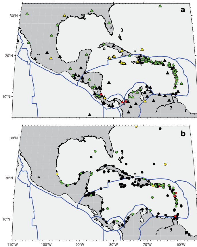
FIGURE 6. ICG/CARIBE-EWS (a) seismic and (b) sea level station data availability maps for October 2021. These maps provide a snapshot of the percent data available from the seismic and sea level stations that the NOAA Pacific Tsunami Warning Center, the Regional Tsunami Service Provider, received in a timely fashion (within 15 minutes) for tsunami warning. Blue lines show tectonic plate boundaries where earthquakes are likely to occur. The colored triangles (a) and dots (b) represent the percent of data available: green >90%, yellow >50%–89%, red >0%–49%, and black, no data received.
