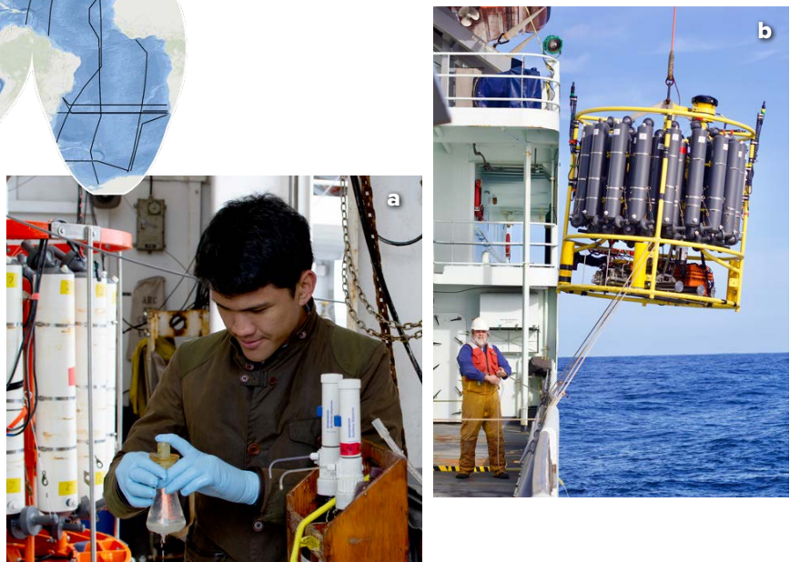
FIGURE 4. (a) Sampling for oxygen during GO-SHIP 108S on R/V Roger Revelle in 2016. Photo credit: Earle Wilson (b) A CTD/rosette package is launched during GO-SHIP 106S aboard R/V Thomas Thompson in 2019. Photo credit: Isa Rosso
