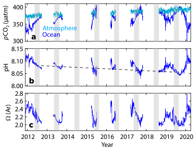
FIGURE 2. Time series of (a) measured surface ocean and atmospheric CO 2 partial pressure ( p\text{CO}_2 ), (b) calculated pH, and (c) calculated carbonate saturation state ( \Omega ) at SOTS between late 2011 and early 2020; gray shading indicates the winter (JJA) season. The black dashed line is a simple regression between the 2012 and 2019 winter pH data—quantification of trends in the deseasoned data is the focus of ongoing work.
