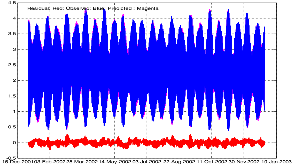
Figure 4: Graphs of observed (blue), predicted (magenta) and residual (red) using 2002 hourly sea level data for Lamu by T_TIDE.
