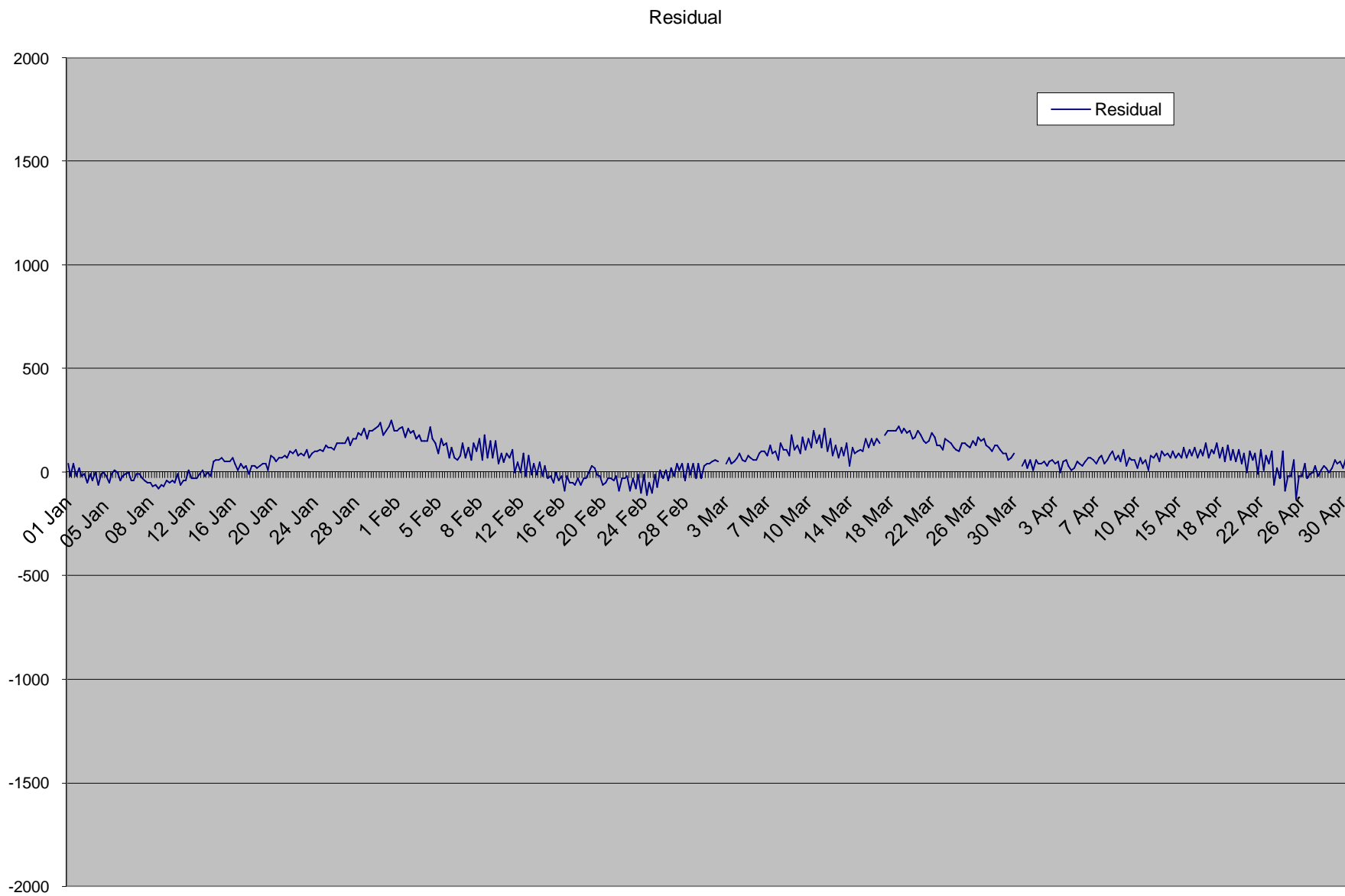
Figure 13: Graph showing residual plot (mm) for Rodrigues station from January to April 2008 (by SLPR2).
