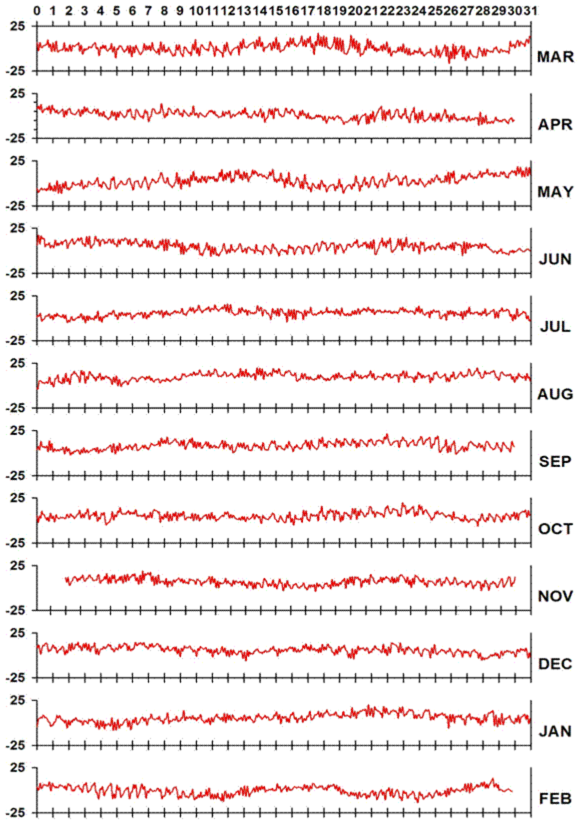
Fig. 8: Plot of Residual Sea Levels (mm) in Zanzibar for March 2007 to February 2008 by SLPR2
