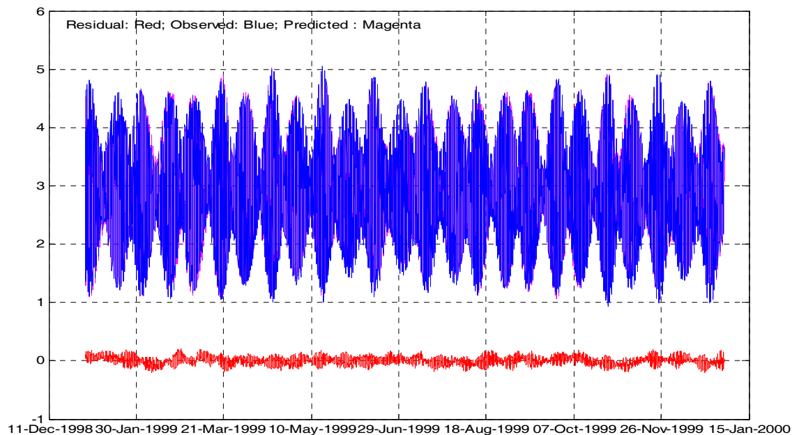
Figure 3: Graphs of observed (blue), predicted (Magenta) and residual (red) using 1999 hourly sea level data for Mombasa by T_TIDE.
