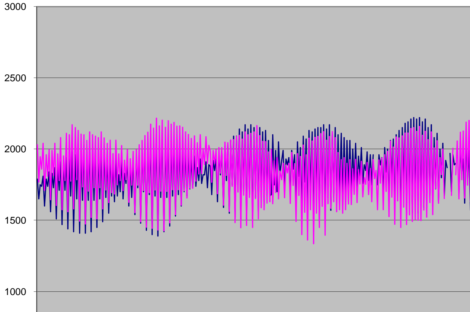
Figure 10: Graph showing Observed v/s Predicted (mm) for Port Louis tide data from 01 January to April 2008 (by SLPR2)
