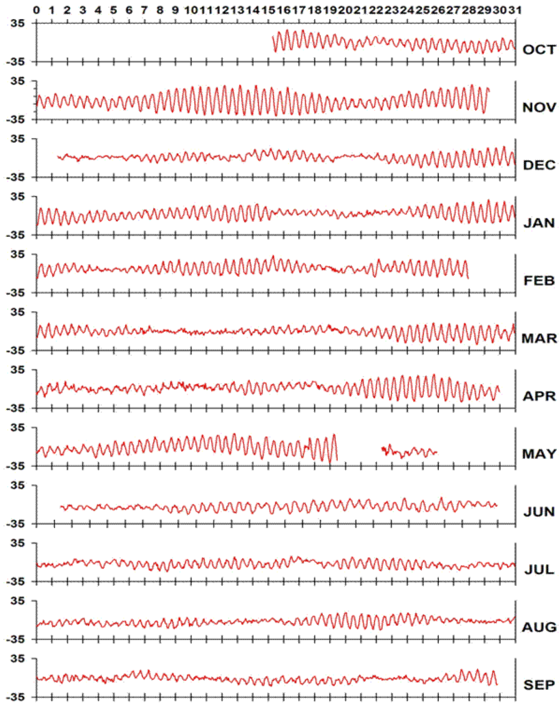
Figure 9: Plot of Residual Sea Levels in Dar es Salaam for October 1989 to September 1990 by SLPR2
